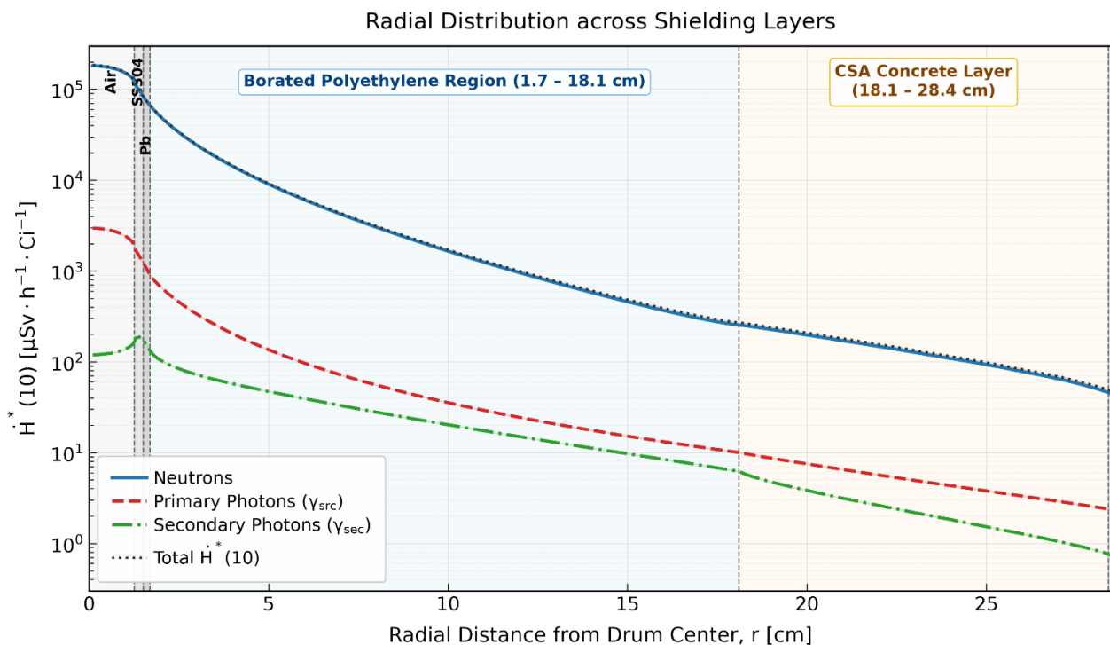
Figure 6: Radial ambient dose equivalent rate profiles for neutrons, primary photons ( \gamma_{src} ), secondary photons ( \gamma_{sec} ), and total radiation across concentric shielding layers of the optimized drum configuration.
