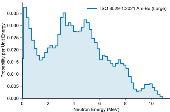
Figure 3: Energy spectrum of the Am-Be neutron source as defined by the ISO 8529-1:2021 standard (ISO 2021), utilized as the source definition in the Monte Carlo simulations.
