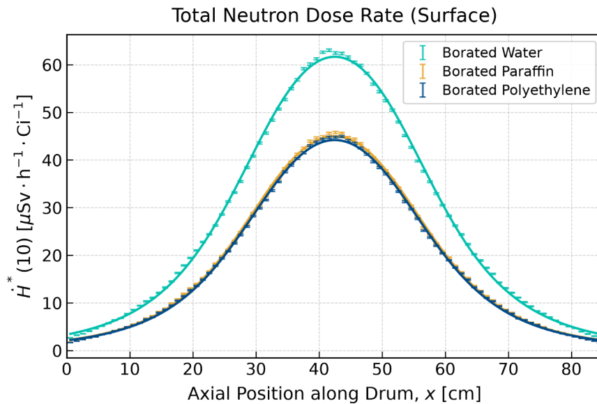
Figure 4: Superimposed empirical model fittings of the neutron ambient dose equivalent rates at the surface.
