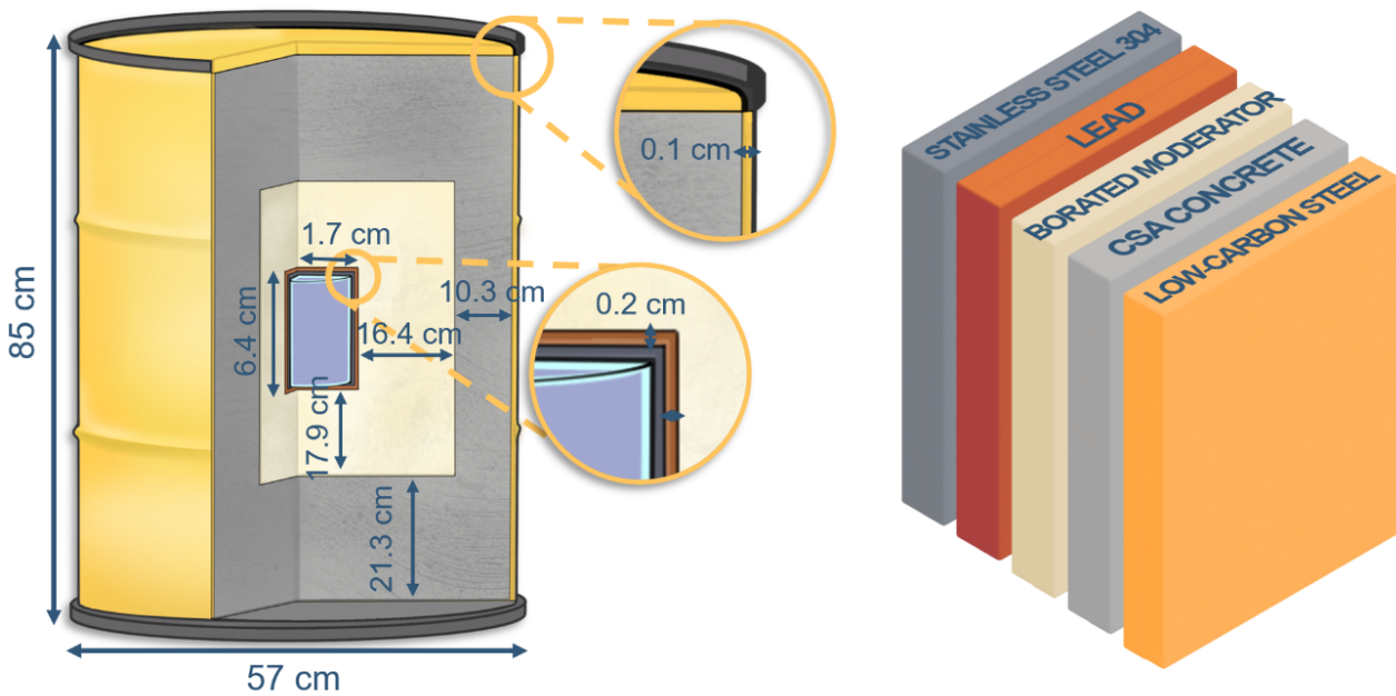
Figure 2: Cross-sectional geometry and dimensions of the shielding drum model.
