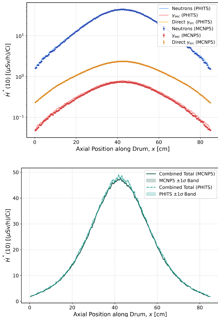
Figure 9: Comparison of PHITS 3.35 and MCNP5 axial ambient dose equivalent rate profiles for the optimized shielding drum: (top) primary neutrons, secondary capture gamma rays, and source gamma rays; (bottom) total ambient dose equivalent rate with \pm 1\sigma uncertainty bands.
