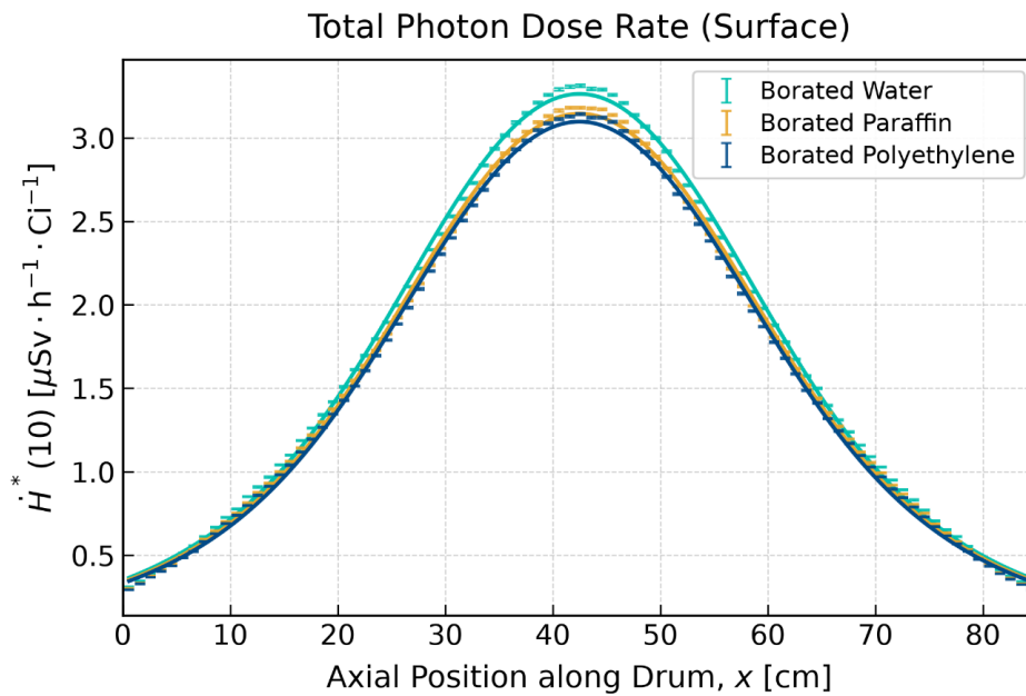
Figure 5: Superimposed empirical model fittings of the photon ambient dose equivalent rates at the surface.
