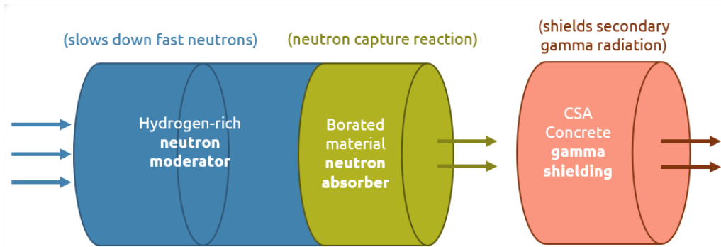
Figure 1: Neutron-shielding framework
