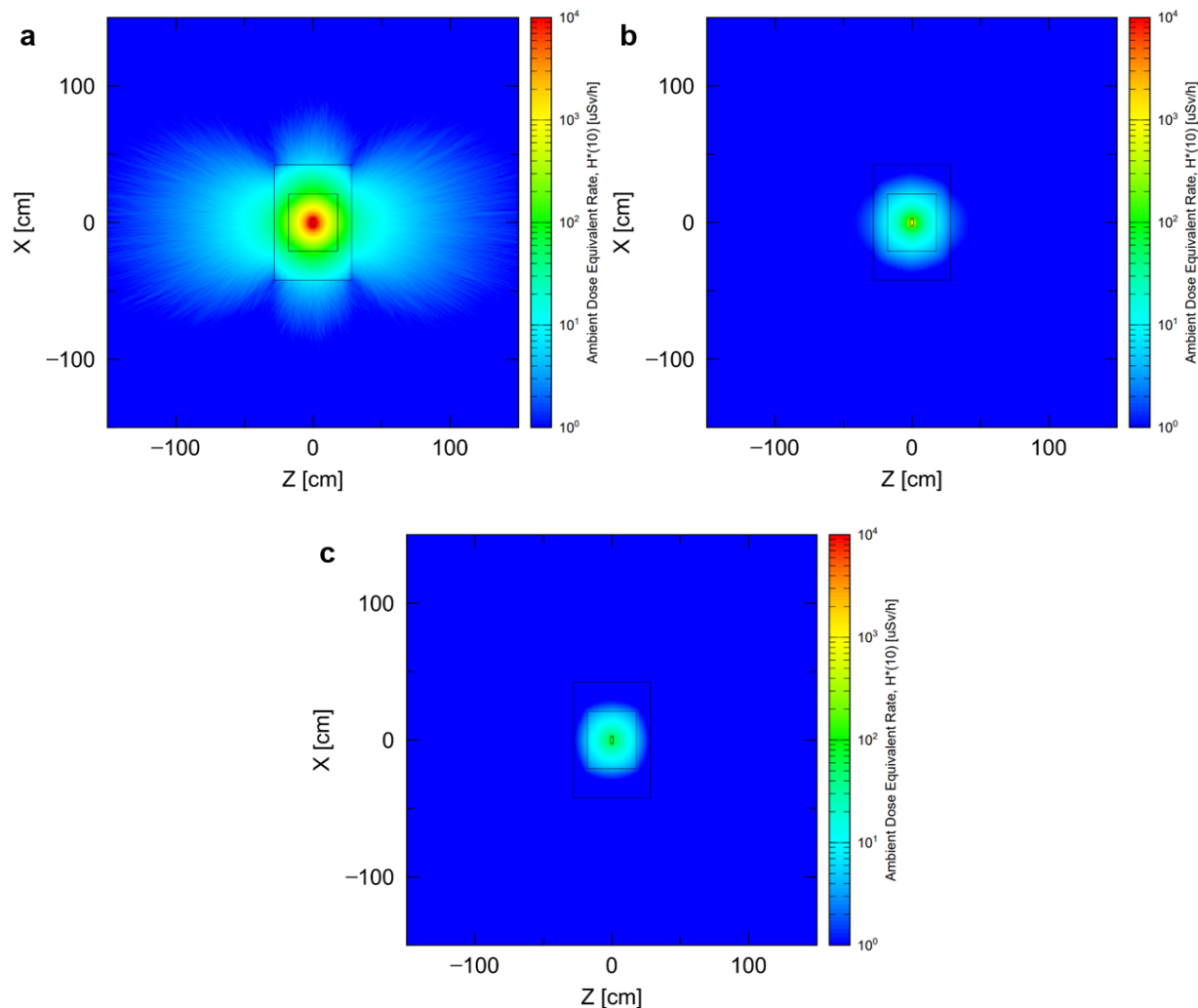
Figure 7: Cross-sectional 2D heatmaps of the (a) neutron, (b) primary 4.438 MeV photon, and (c) secondary photon ambient dose equivalent rates ( \mu\text{Sv/h} per Ci ^{241}\text{Am-Be} source) for the optimized shielding configuration consisting of borated polyethylene and CSA-based concrete layers.
