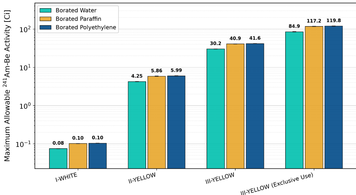
Figure 8: Maximum allowable ^{241}\text{Am-Be} source activity (Ci) across IAEA SSR-6 transport package categories (Category I-WHITE, Category II-YELLOW, Category III-YELLOW, and Category III-YELLOW Exclusive Use) for shielding drum configurations utilizing borated polyethylene, borated paraffin, and borated water moderators.
